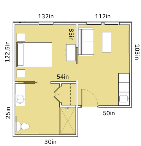
Ash Floor Plan 377 SQ.FT. 10 UNITS
